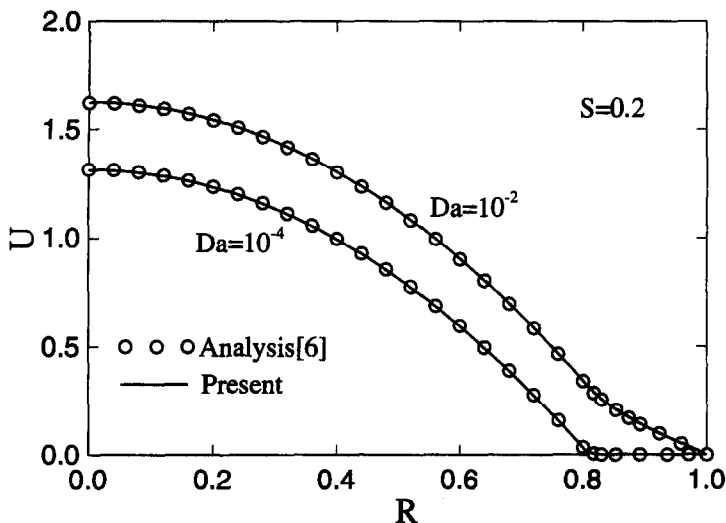
Fig. 2. Comparison of steady non-pulsating velocity profile. S = 0.2 , B = 0.32 .
